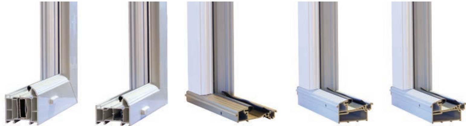
77mm uPVC Full Frame Threshold Distance from bottom of door leaf to bottom of threshold - 48mm
